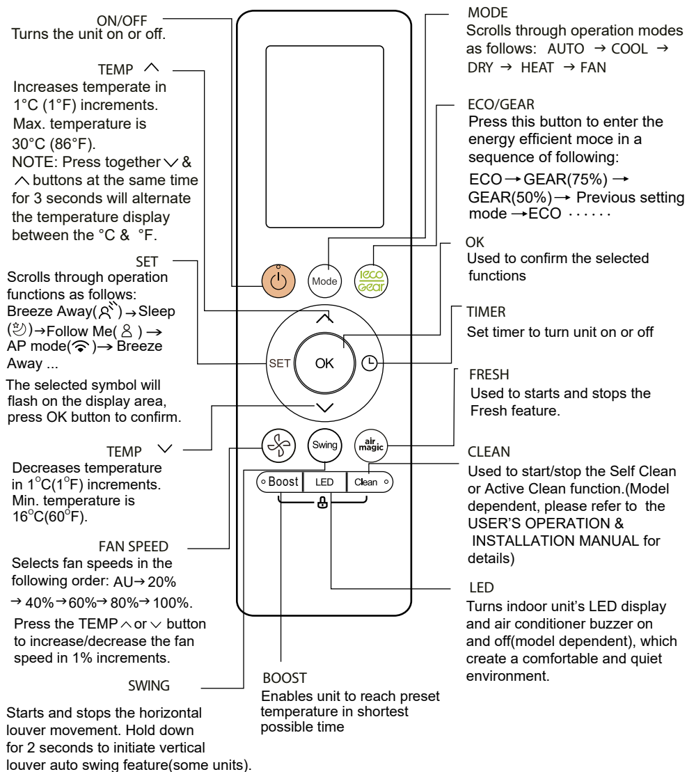
Model: RG10A1(B2S)/BGEF
