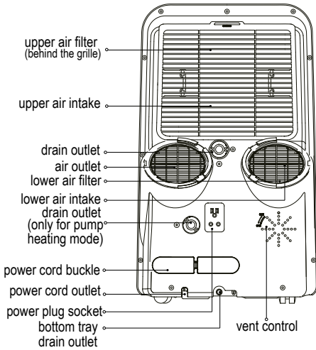
rear
